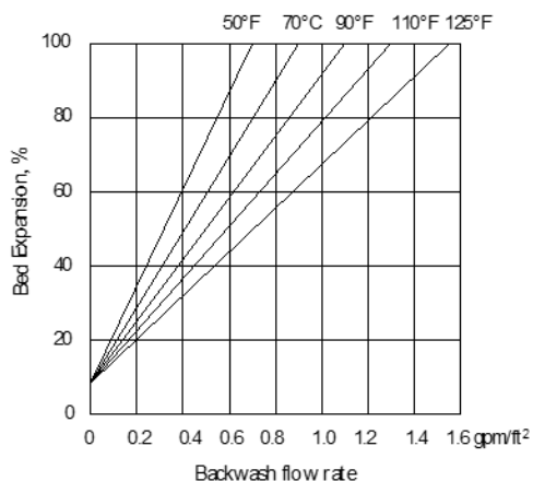
Figure 1: Backwash Expansion
