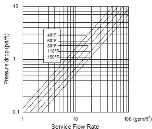
Figure 2: Pressure Drop
