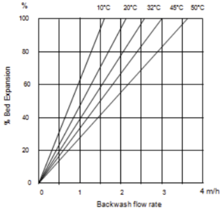
Figure 1: Backwash Expansion
