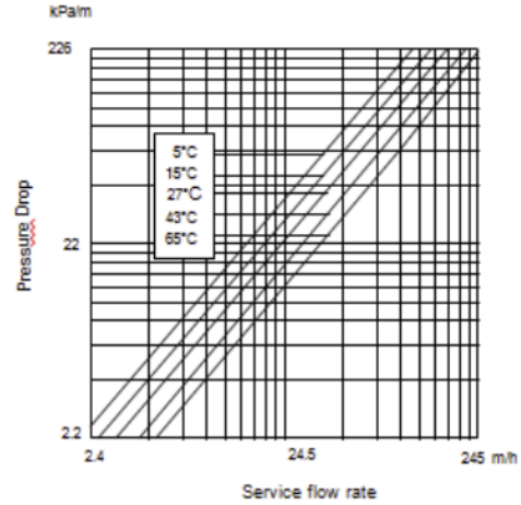
Figure 2: Pressure Drop
