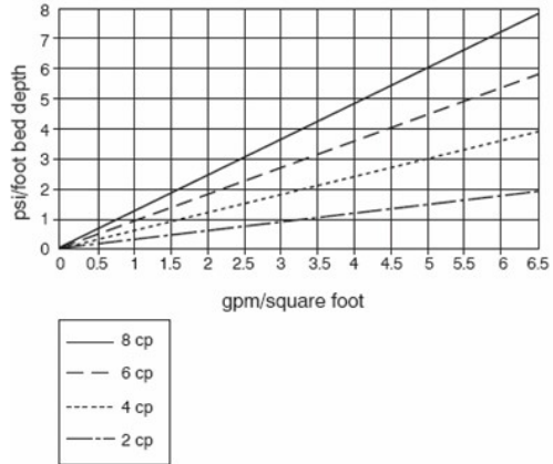
Figure 1: Pressure Drop
