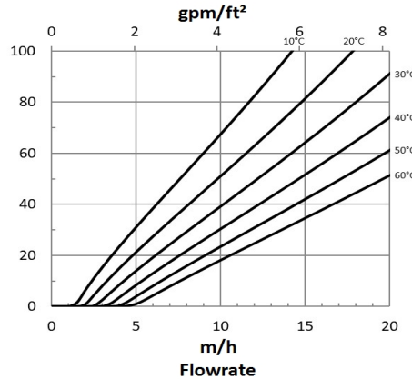
Figure 1: Backwash Expansion Temperature = 10 – 60°C (50 – 140°F)
