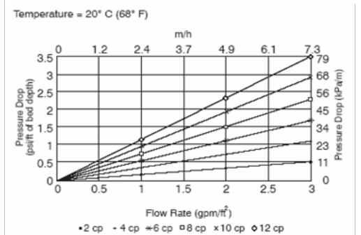
Figure 2: Pressure Drop
